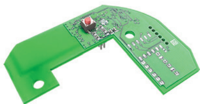
FUNKMODUL BASIS X
